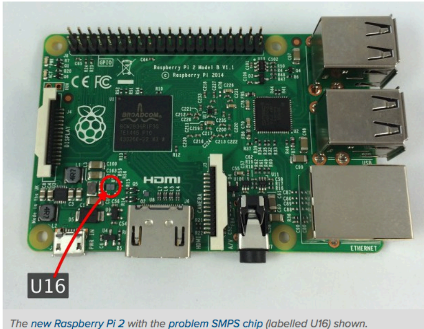
The new Raspberry Pi 2 with the problem SMPS chip (labelled U16) shown.
